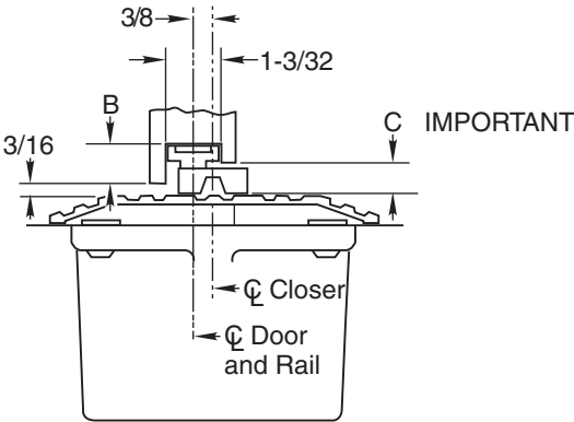
WITH THRESHOLD Set Cement Case Flush with Finished Floor Closer must have a 1/2" longer spindle for threshold.
