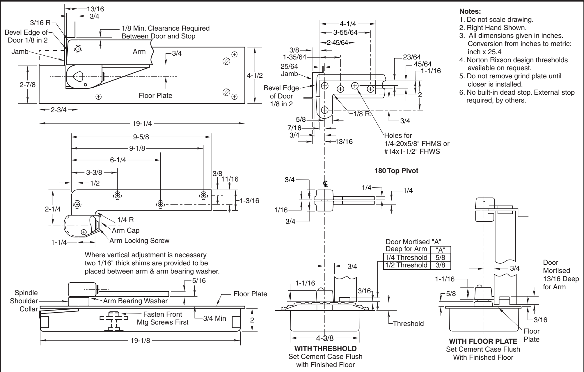
51 Floor Closer 3/4" Offset
