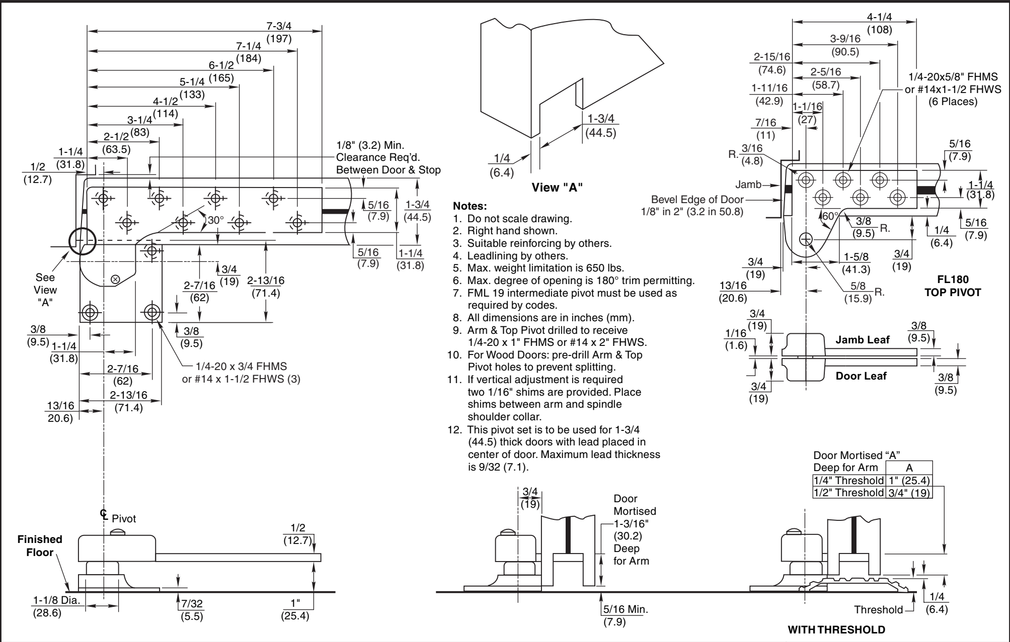
FL147 Pivot Set 3/4" Offset For 1-3/4" Lead Lined Fire Doors
