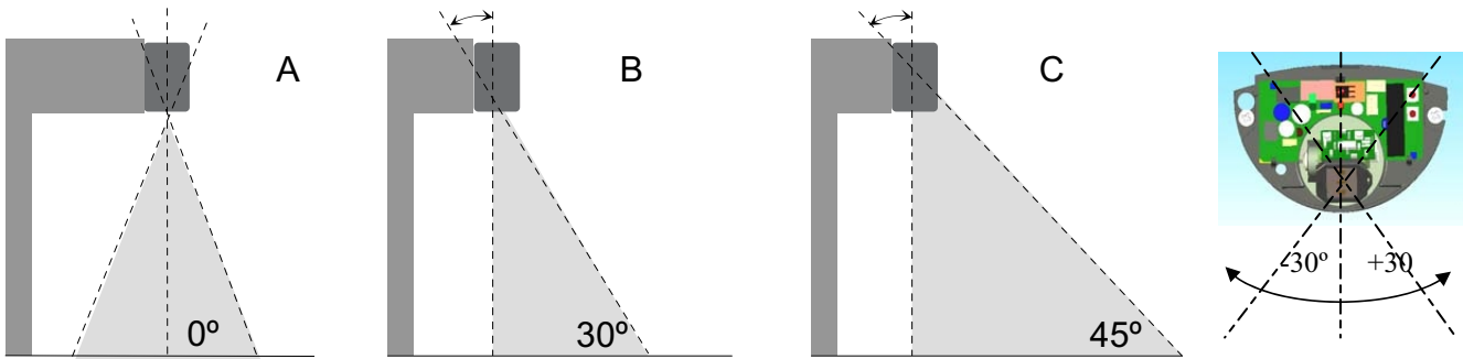
Sensing field as close to the door as possible: -antenna set at the position of 0° Sensing field close to the door: -antenna set at the position of 30° Sensing field far from the door: -antenna set at the position of 45°
