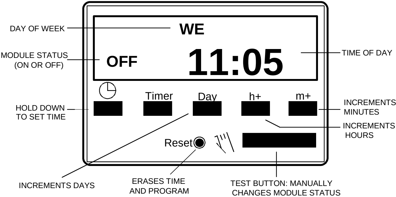
DISPLAY MODULE: PROGRAMMING MODE
