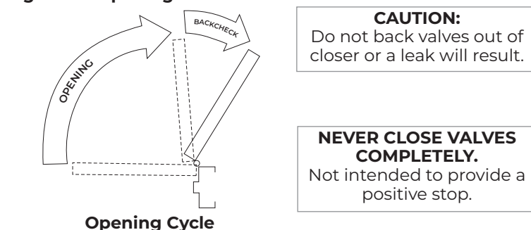
Figure 4 - Opening Door Control
