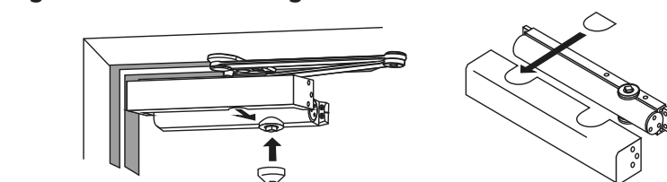
Figure 6 - Cover Mounting
