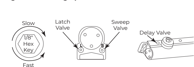
Figure 3 - Closing Power Controls
