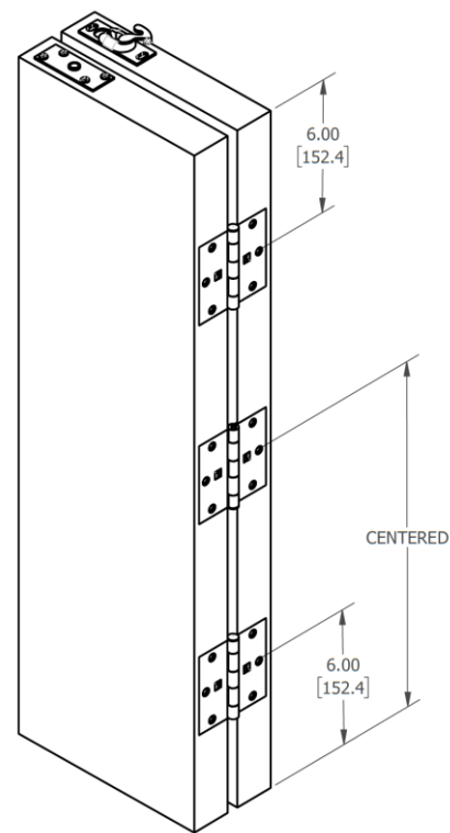
Figure 6: Hinge Locations
