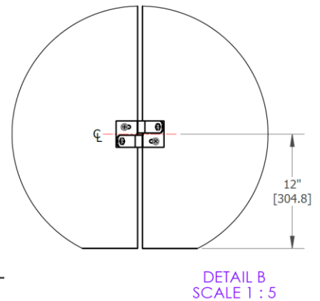
Figure 9: 4-Panel Bi-Fold Aligner Location
