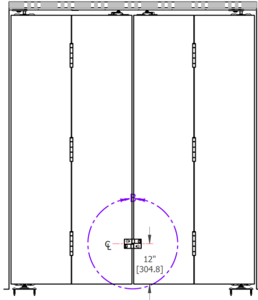
Figure 9: 4-Panel Bi-Fold Aligner Location
