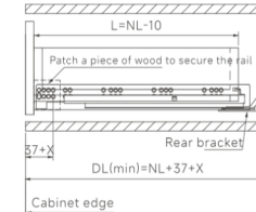
Inset drawer
