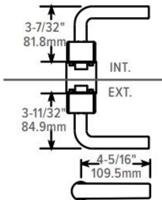
2190 WITH ME LEVER
