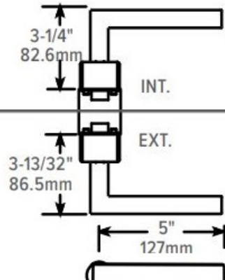
2190 WITH MI LEVER
