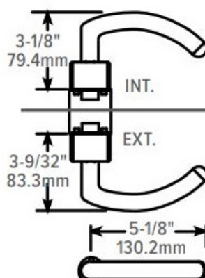
2190 WITH MG LEVER
