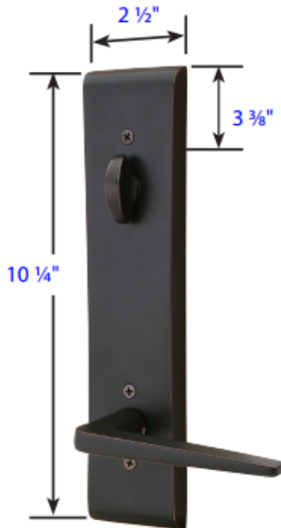
Standard interior trim Part # 4815 & 4816
