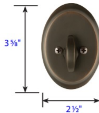
Interior Trim (8458)
