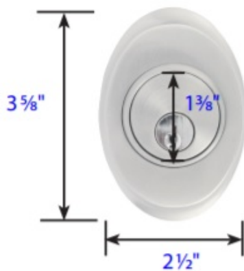
Exterior Trim (8458)
