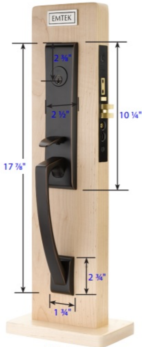
Artemis Trim Style Part # UL 3344
