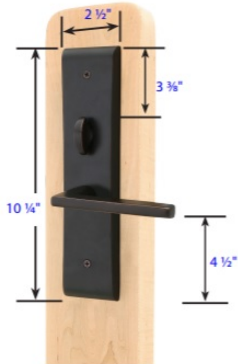
Standard interior trim Part # UL 3344 & 3345
