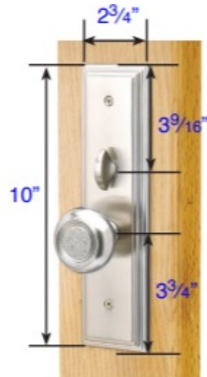
Standard interior trim Part # UL 3310, 3306 & 3305
