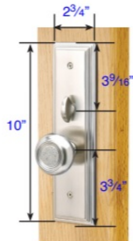
Standard interior trim Part # UL 3310, 3306 & 3305
