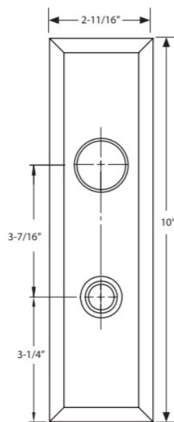
Outside Trim
