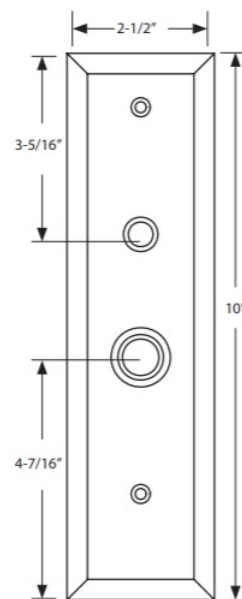
Inside Trim
