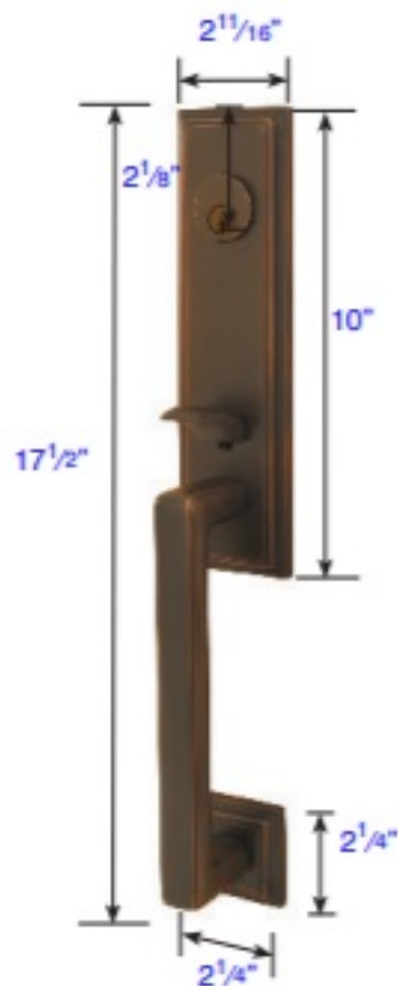
Wilshire Style Part # 4211
