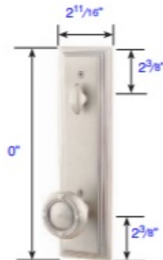
Standard interior trim Part # 4211 & 4212
