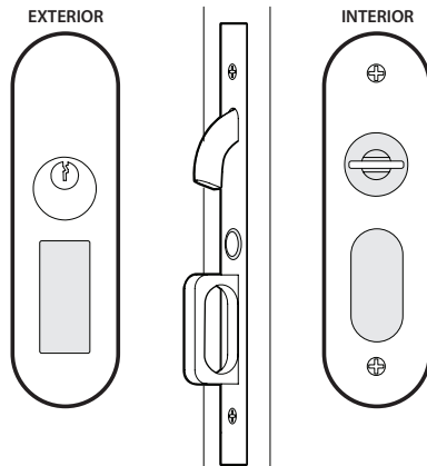
Keyed Pocket Door Mortise Lock
