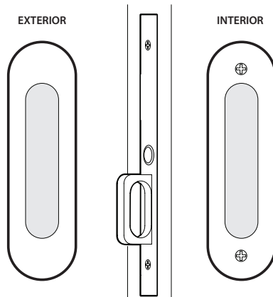
Passage Pocket Door Mortise Lock
