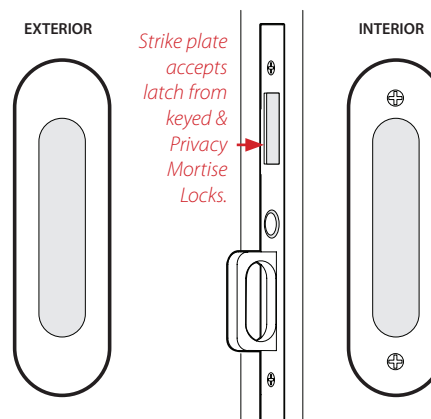
Dummy Pocket Door Mortise Lock
