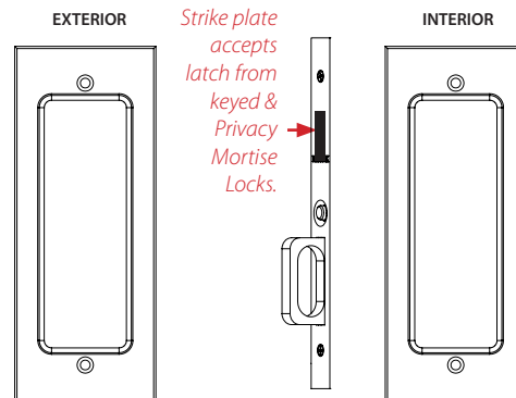
Dummy Door Mortise Lock
