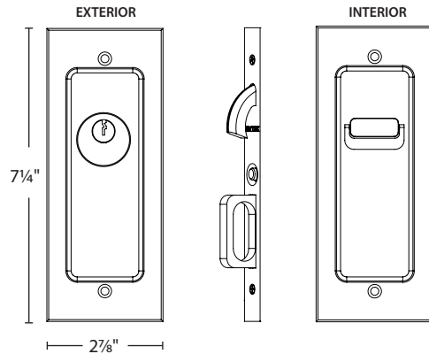
Keyed Door Mortise Lock
