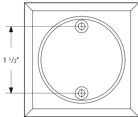
TUBULAR POCKET SQUARE ROSETTE PASSAGE, INSIDE TRIM
