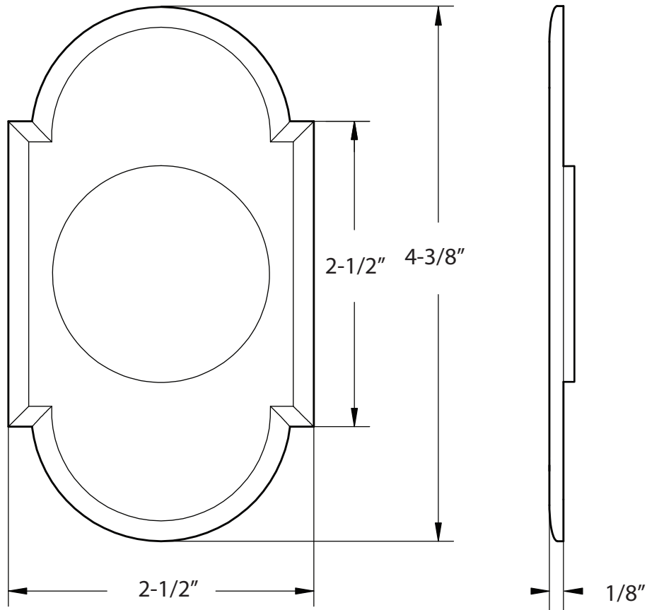
#8 TUBULAR POCKET PASSAGE, OUTSIDE TRIM
