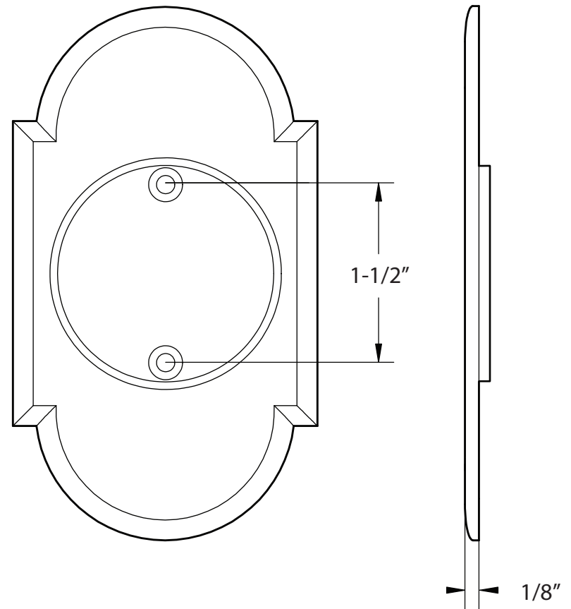
#8 TUBULAR POCKET PASSAGE, INSIDE TRIM
