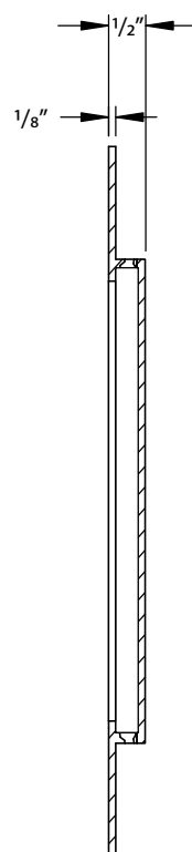
CROSS SECTION
