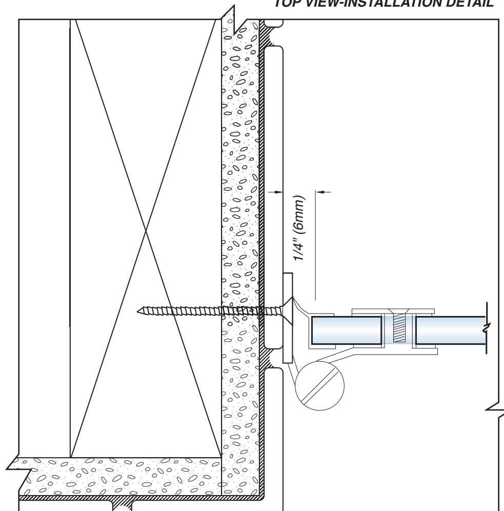
TOP VIEW-INSTALLATION DETAIL
