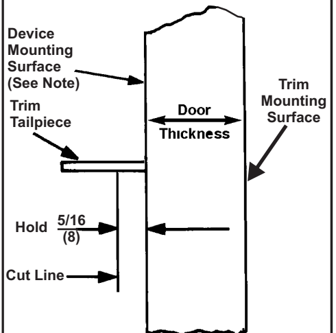
Figure 2: Tailpiece Sizing
