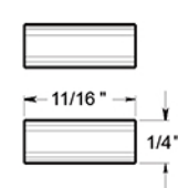
(X2) RAISED INSTALLATION SPACERS
