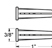
(X2) PLASTIC ANCHORS
