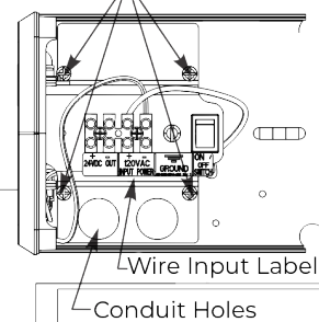
Conduit Assembly Mounting Screws
