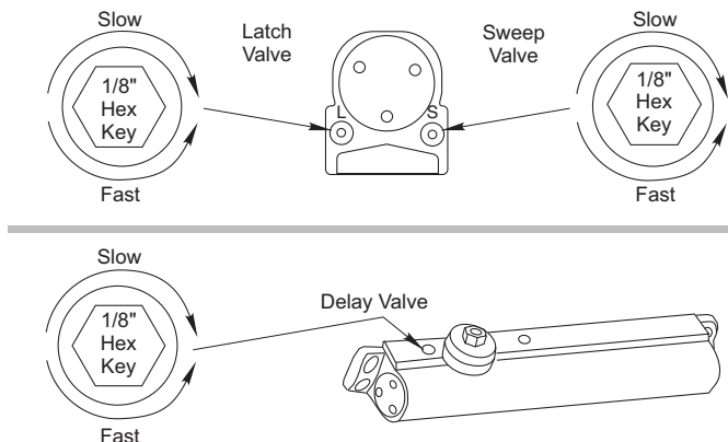
Delayed Action Closing Cycle 3B
