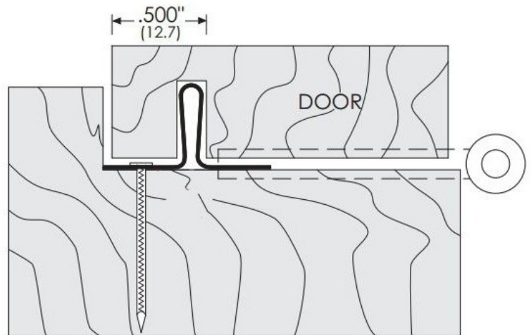
HINGE-SIDE JAMB
