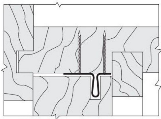
HEAD AND SILL
