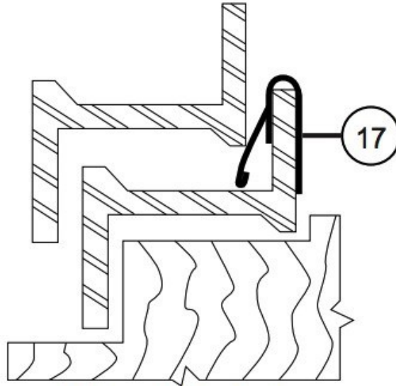
Hinge-Side Jamb
