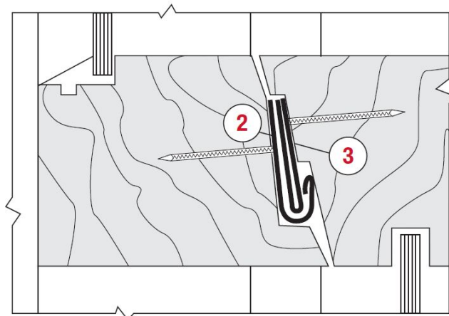
MEETING RAILS
