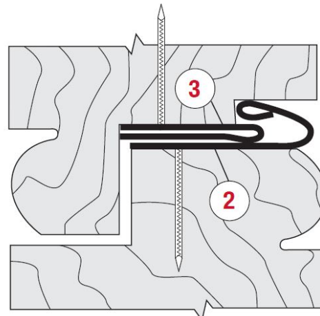
MEETING STILES
