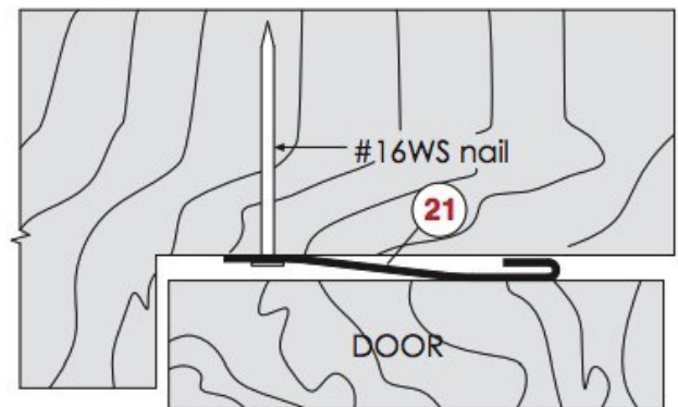
HINGE-SIDE JAMB
