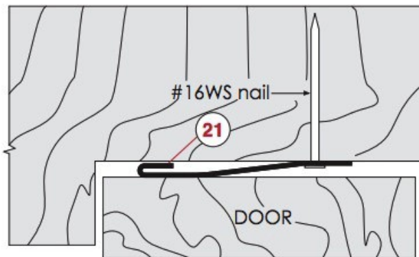
HEAD & LOCK-SIDE JAMB
