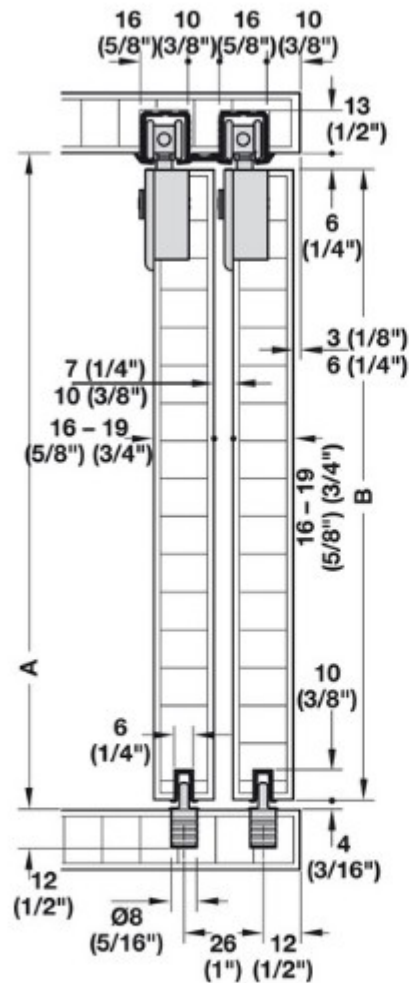
Groove-mounted track
