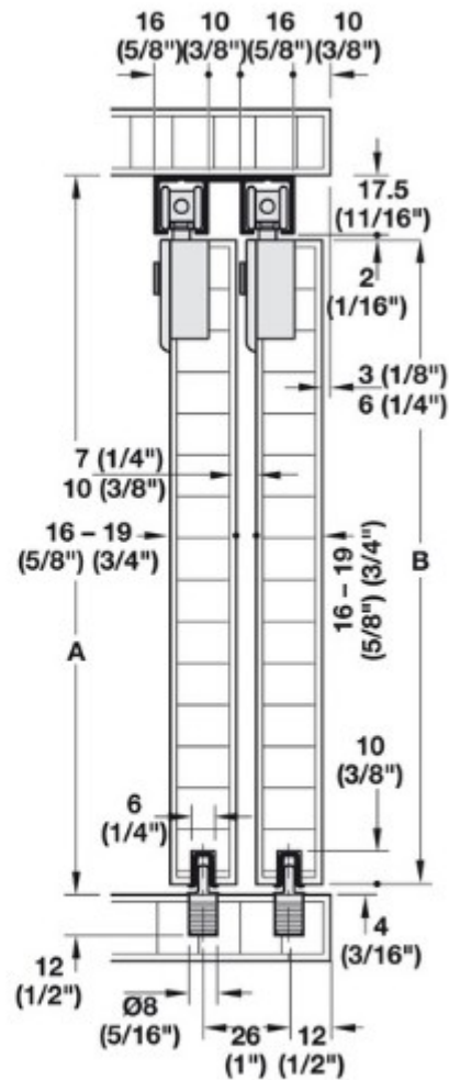
Screw-mounted track
