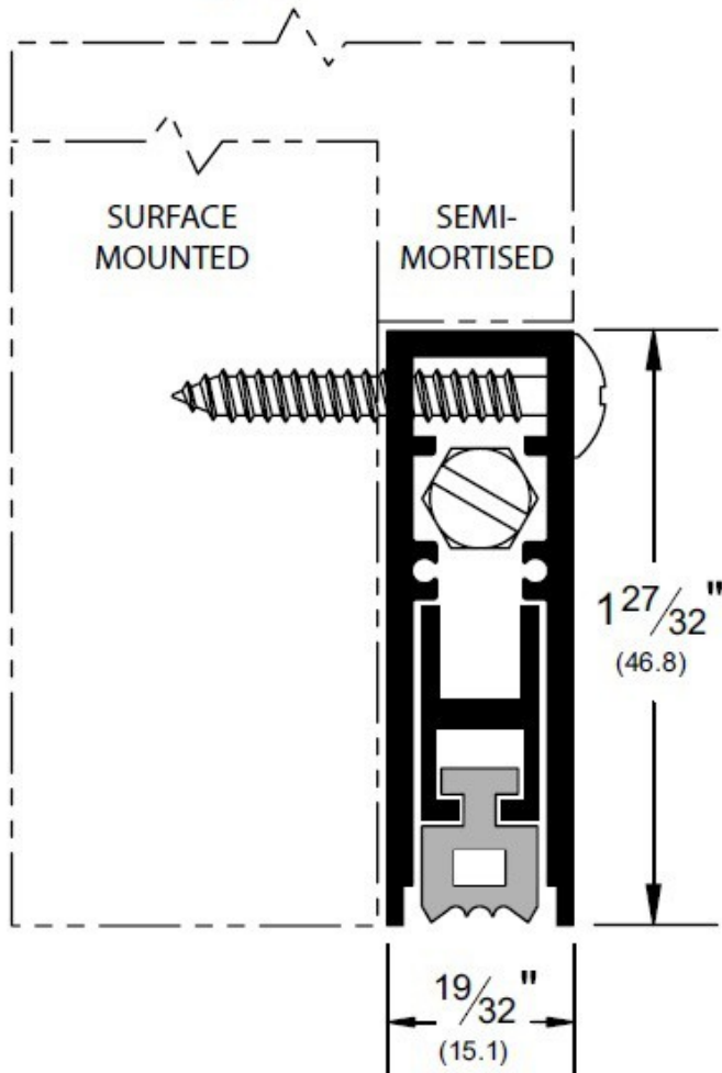
EPDM or Sponge Silicone Seal:
