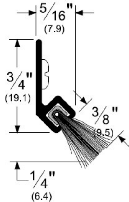
Soft Brush
