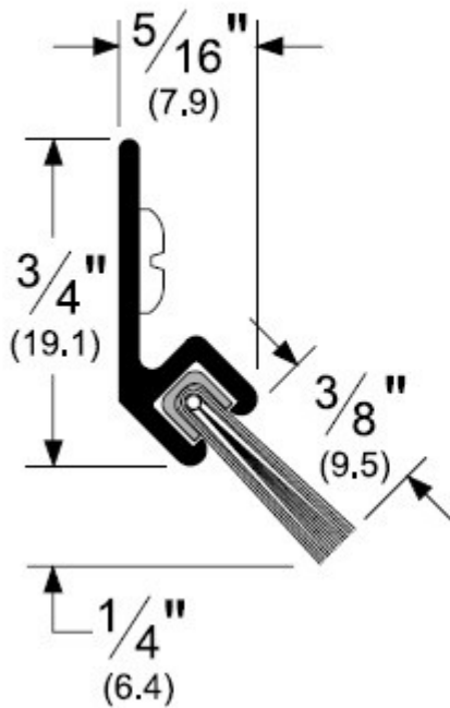
Nylon Brush
