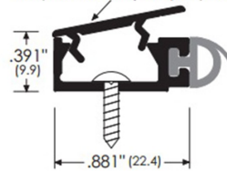
Snap-On Cover (tamper-proof)
