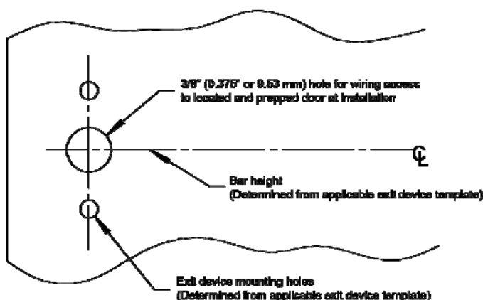
Figure 3. Door Preparation
