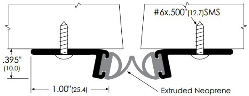
Meeting Stile:
