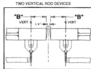
TWO VERTICAL ROD DEVICES VERTICAL ROD x MORTISE DEVICE (OPEN BACK STRIKE REQUIRED FOR MORTISE DEVICE IN THIS APPLICATION)
