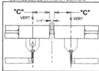
TWO VERTICAL ROD DEVICES VERTICAL ROD x MORTISE DEVICE (OPEN BACK STRIKE REQUIRED FOR MORTISE DEVICE IN THIS APPLICATION)
