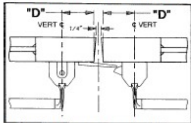
SINGLE DEVICE VERTICAL ROD x RIM DEVICE (571 OR 571A REQUIRED FOR THIS APPLICATION)
