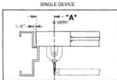
SINGLE DEVICE VERTICAL ROD x RIM DEVICE (571 OR 571A REQUIRED FOR THIS APPLICATION)
