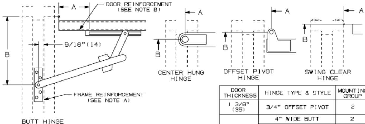
81 SERIES PLAN MOUNTING VIEW LH SHOWN
