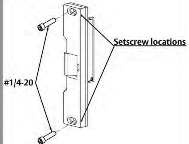
Diagram 3: 1/4" Spacer Removal Diagram 4: Horizontal Adjustability
