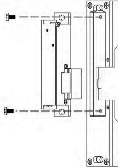
Diagram 2: Faceplate Attachment
