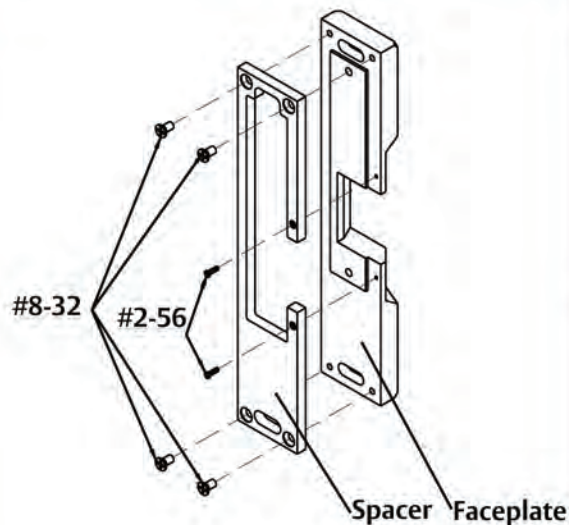
Diagram 3: 1/4" Spacer Removal Diagram 4: Horizontal Adjustability
