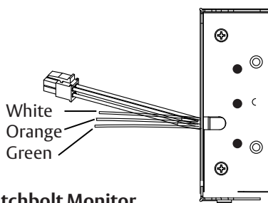
Diagram 3. Latchbolt Monitor
