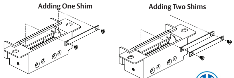
Figure 6: Horizontal Adjustment
