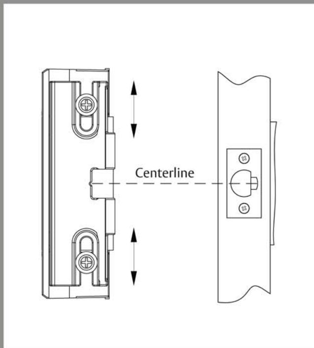
DIAGRAM 7: VERTICAL ADJUSTABILITY
