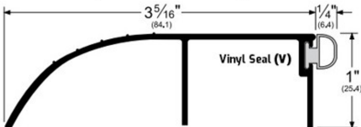
Bumper Threshold with Vinyl Seal
