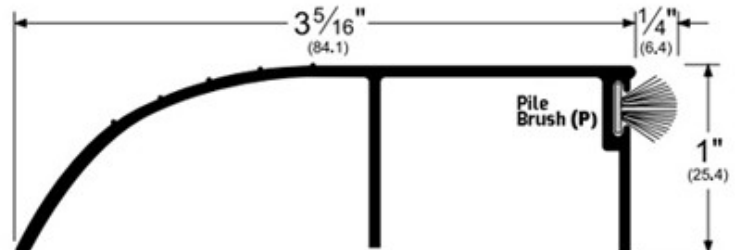
Bumper Threshold with Pile Brush Seal
