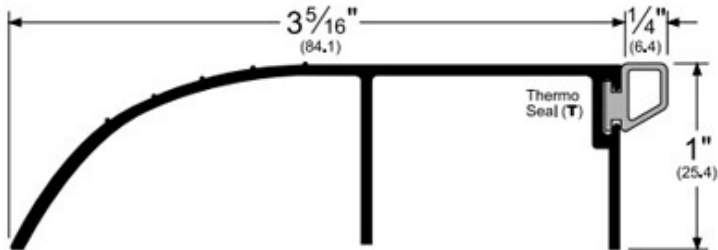
Bumper Threshold with ThermoSeal
