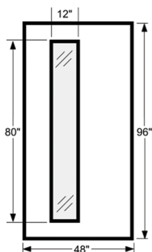
Single Vision Lite, 60-Minute Door
