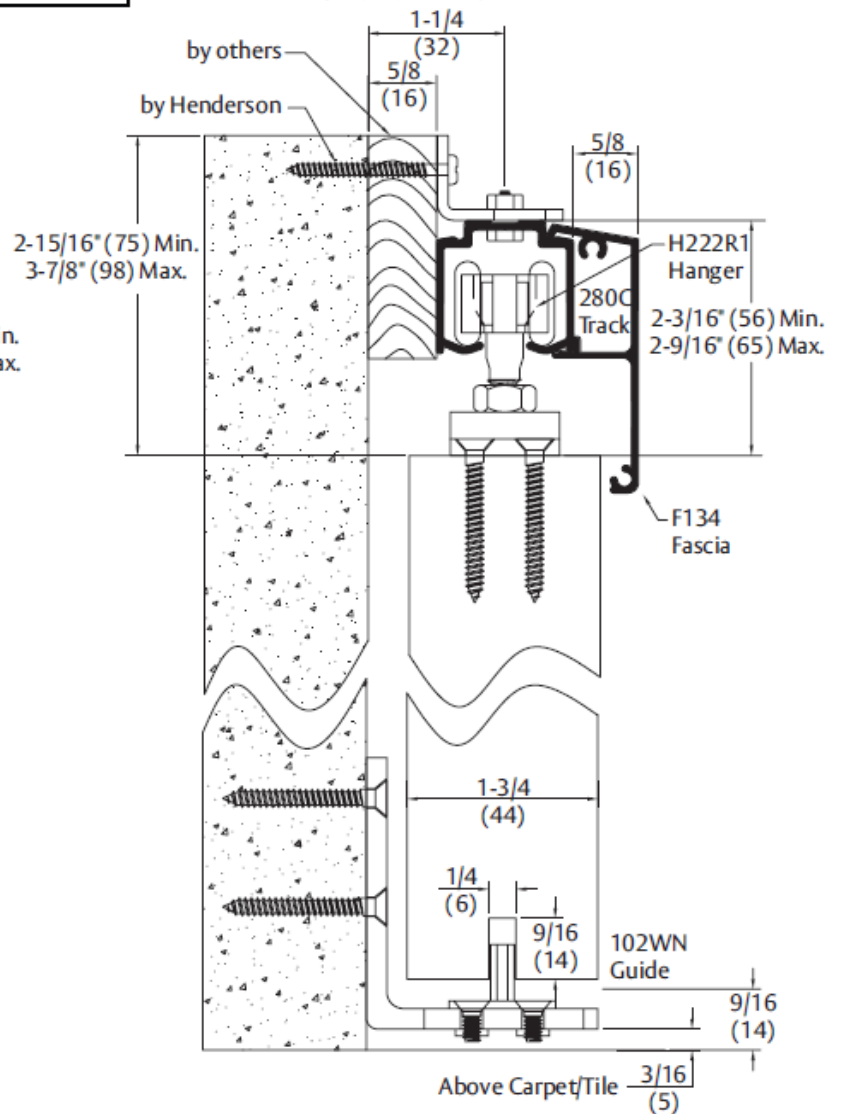
280C Side Wall Mounted 3/4" (19) shim by others
