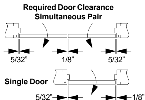
View B: Door Portion
