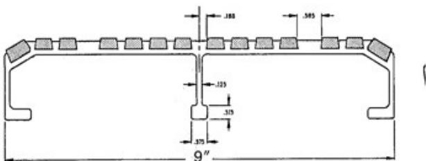
Type I full tread, 9-inch size
