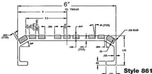
Type I full tread, 6-inch size
