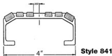
Type I full tread, 4-inch size
