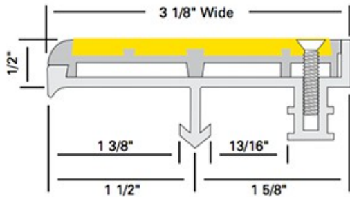
TYPE WP-RN3SP 3 1/8" (79.375 mm) wide 1/2" (12.7 mm) thick
