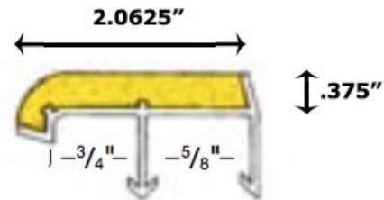
TYPE WP2C
